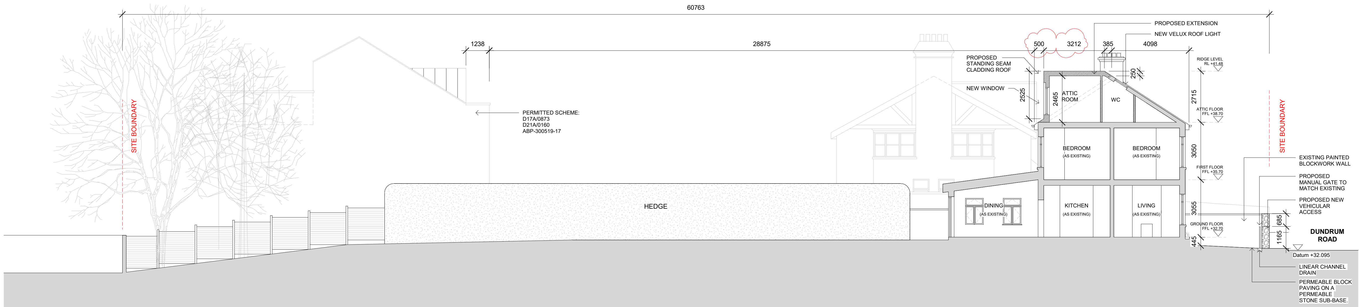
2 PROPOSED CROSS SECTION 1:100
